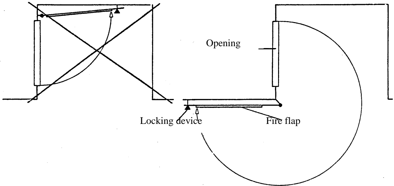
Below deck positioning of a fire flap
