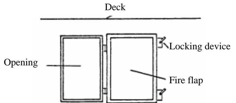
Below deck positioning of a fire flap
