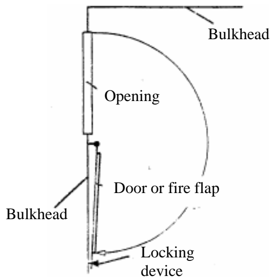
Plan view of a door or fire flap opening on to the open deck
