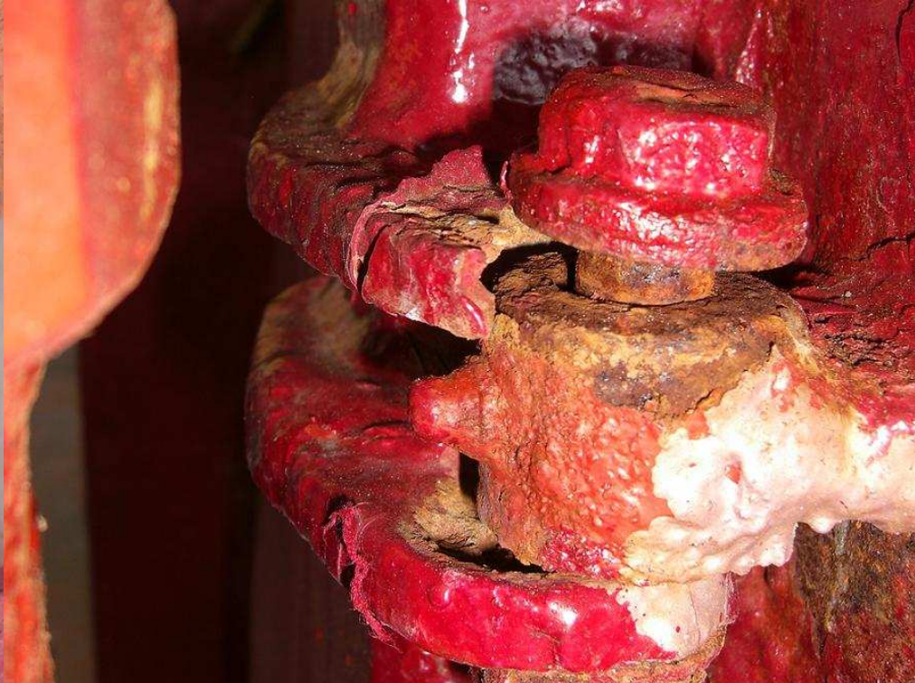
MV Baltic Wind: Decks corrosion, cracking, damaged hatch cover, broken hinges at watertight door, etc.
